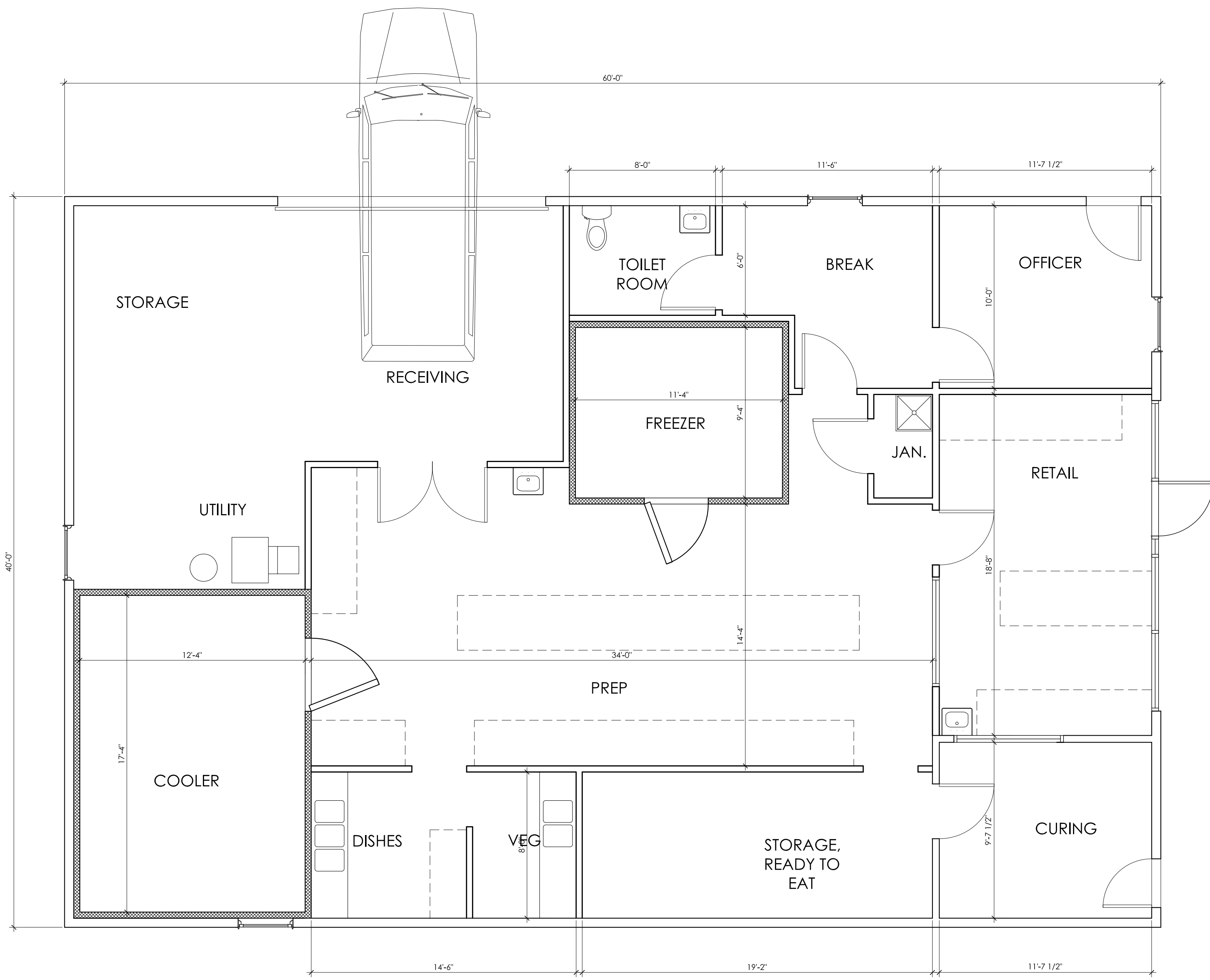
PRELIM FLOOR PLAN ALT 1 SCALE: 1/4" = 1'
